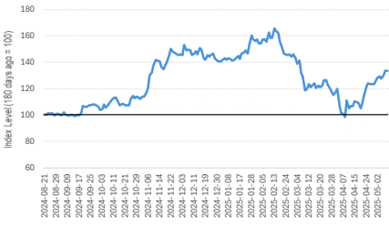
HUBS vs S&P 500 (180 days)
