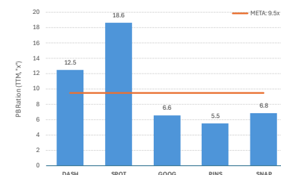
PB ratio
