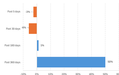
PB ratio
