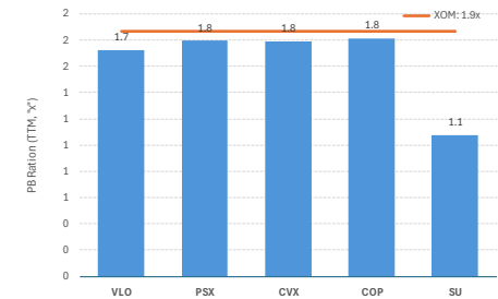
PB ratios
