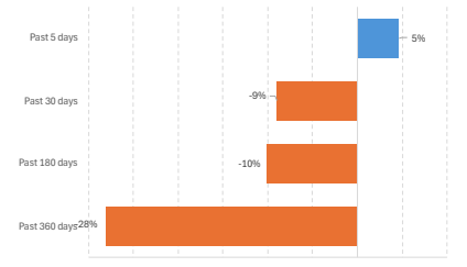
PB ratio
